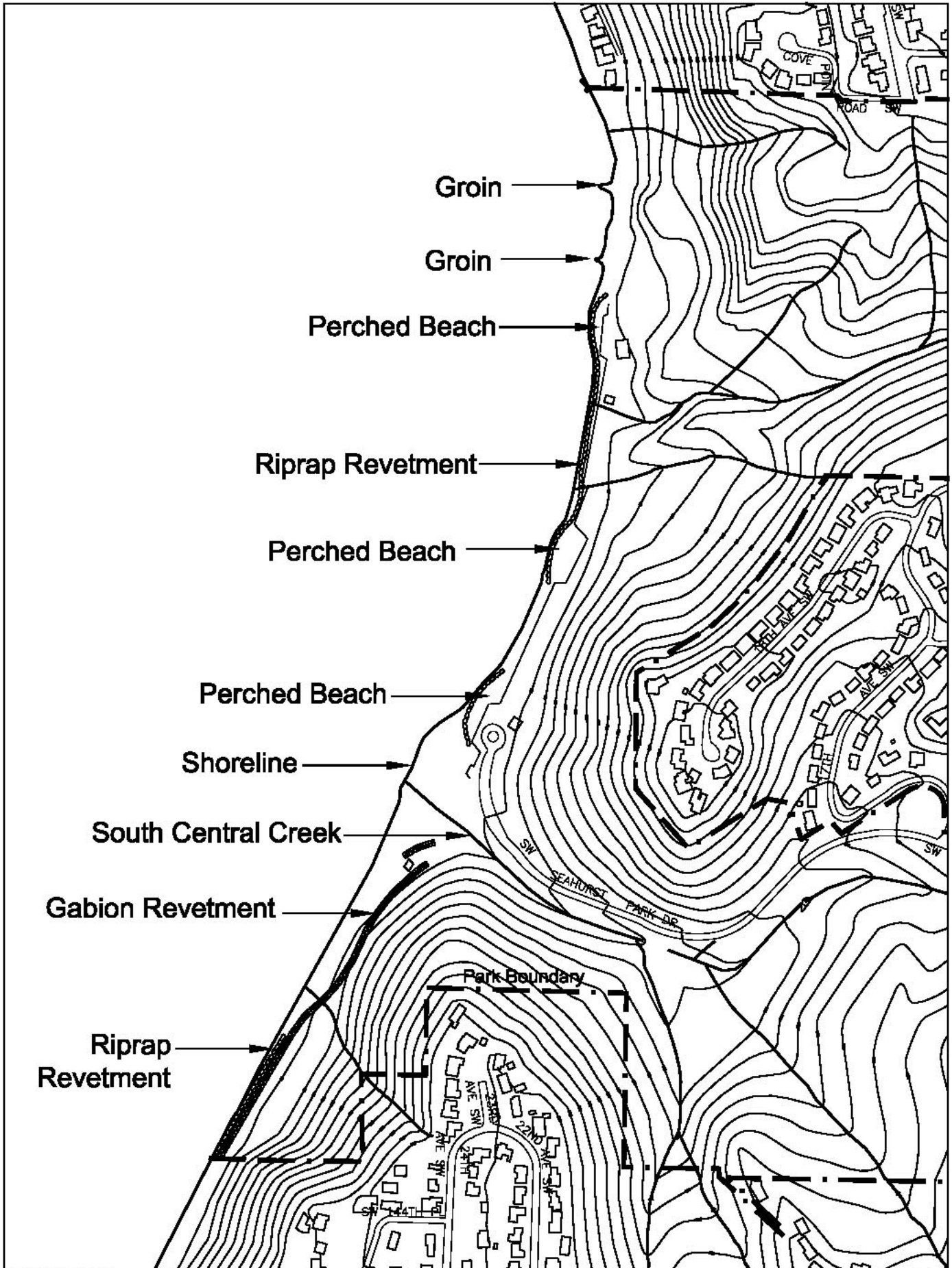
Figure 2 Overview of Shoreline Protection Structures Seahurst Park Master Plan
